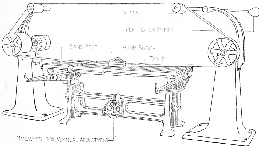
FIG. 204. BELT SANDER.
